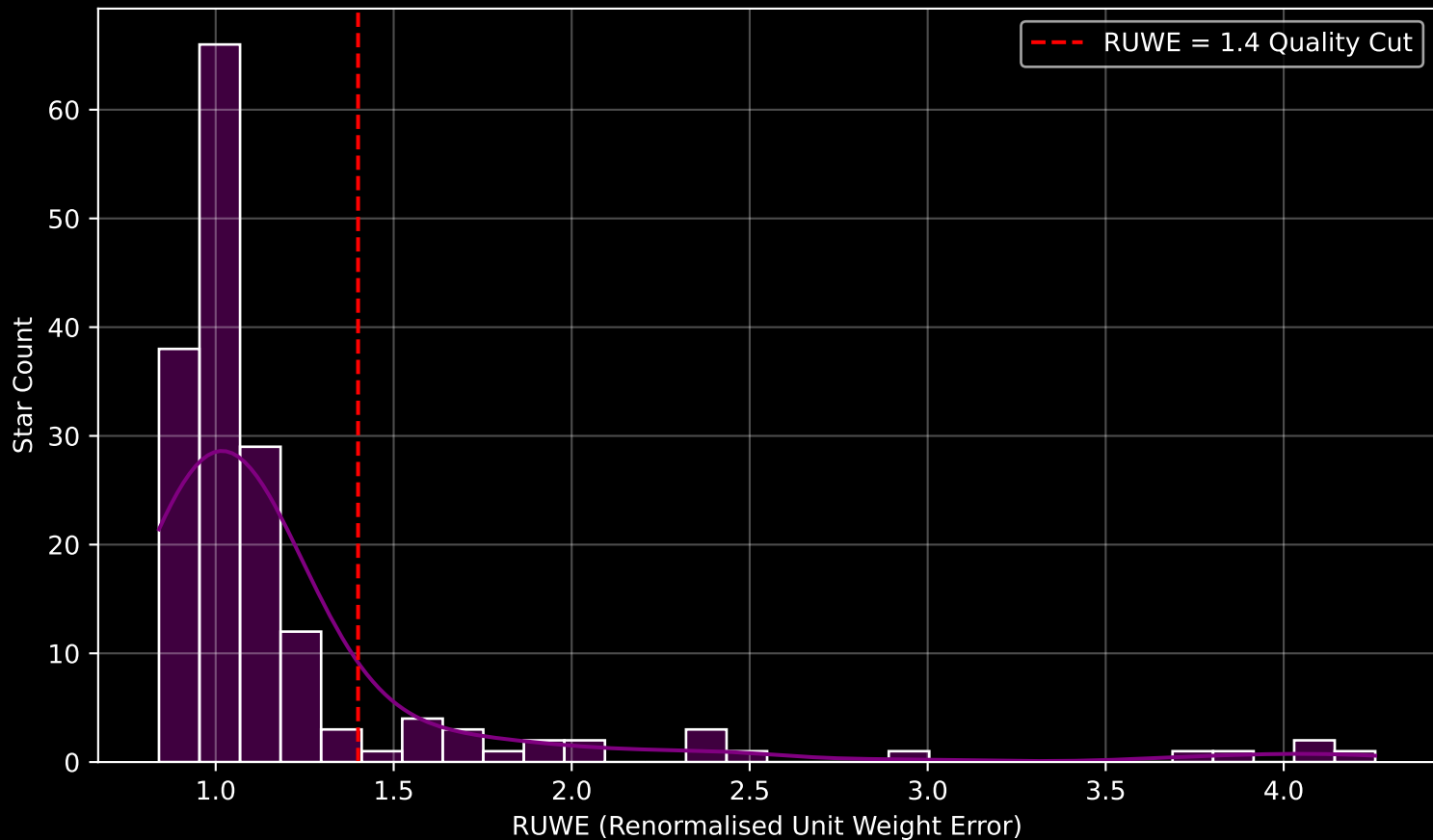
GAPOGEE DR17 Field [037+79_MGA] RUWE Distribution (n= 171)
