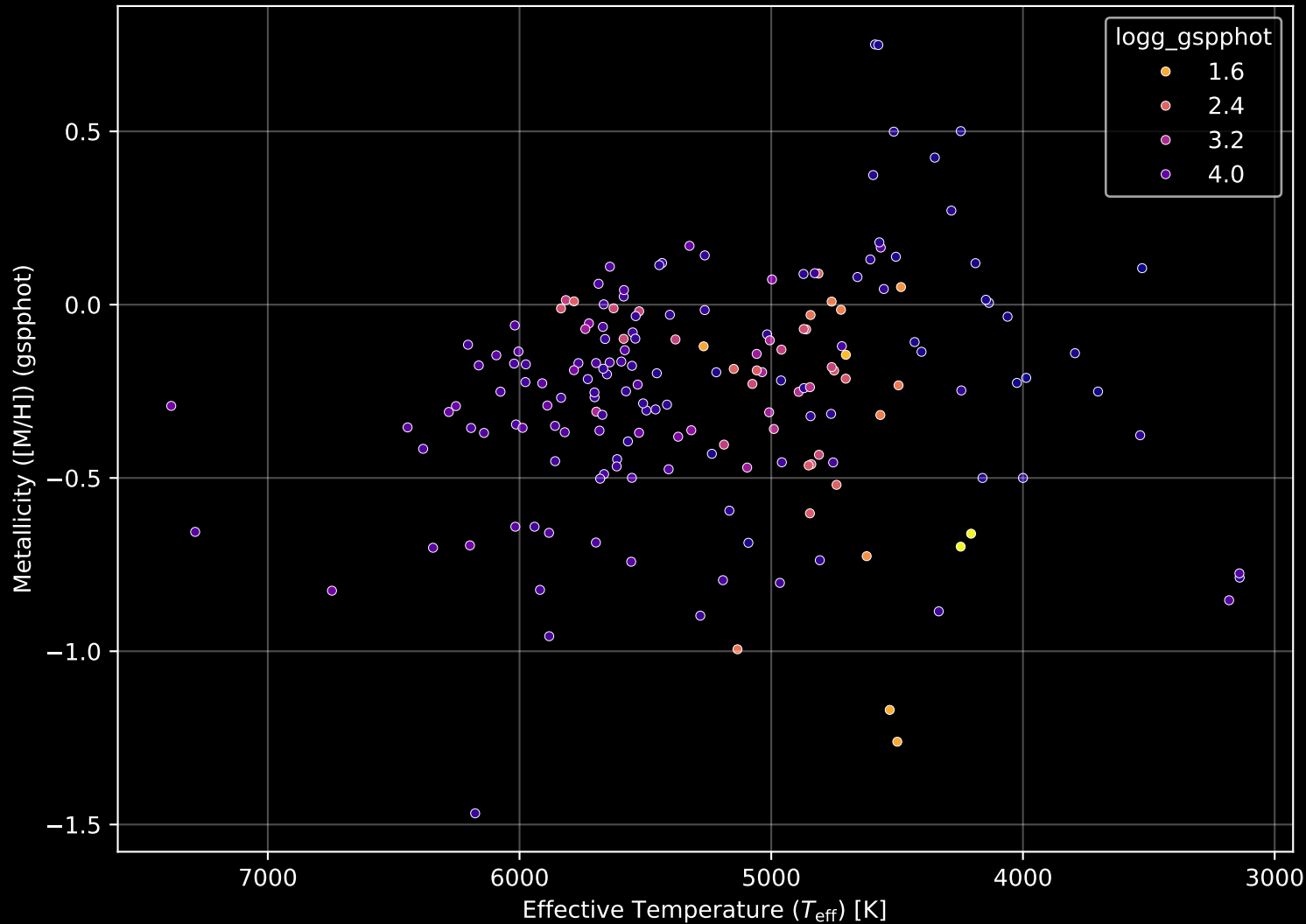
APOGEE DR17 Field: [03+79_MGA] Stellar Population Parameters (n= 182)
