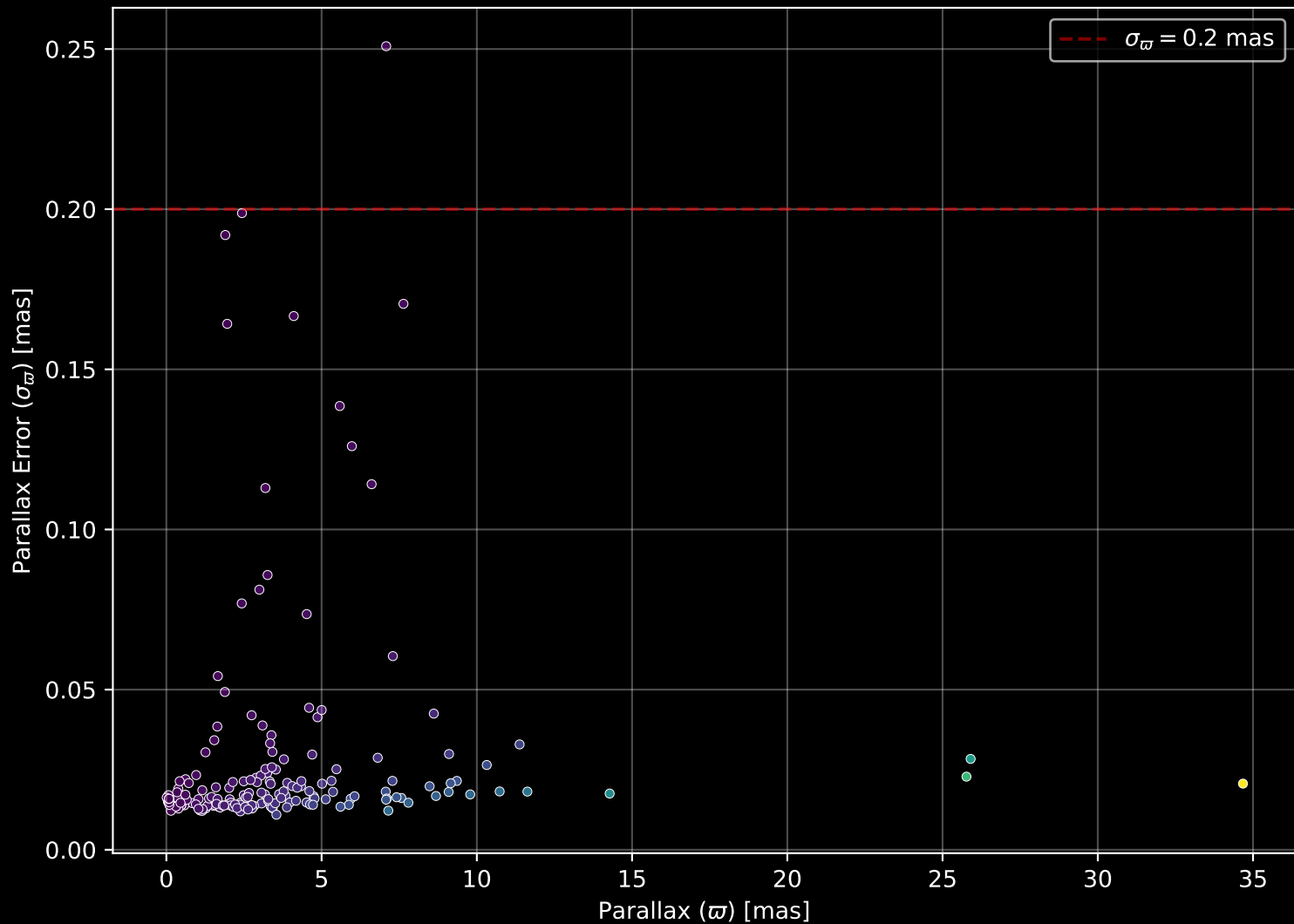
APOGEE DR17 Field: [037+79_MGA] Parallax Quality (n= 182)
