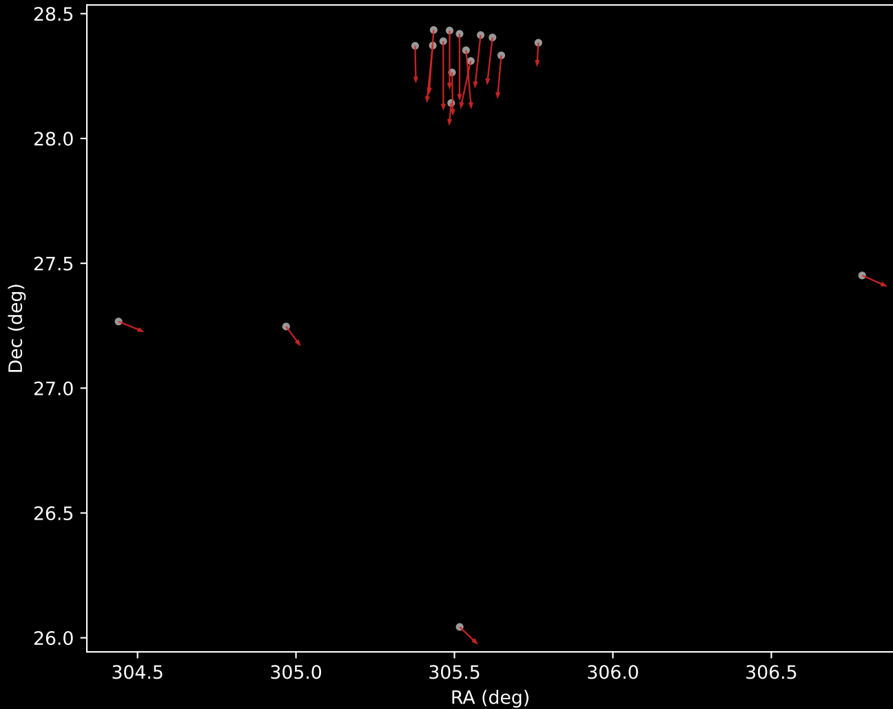
APOGEE DR17 Cluster 6 Proper Motion Vectors (n=18)
