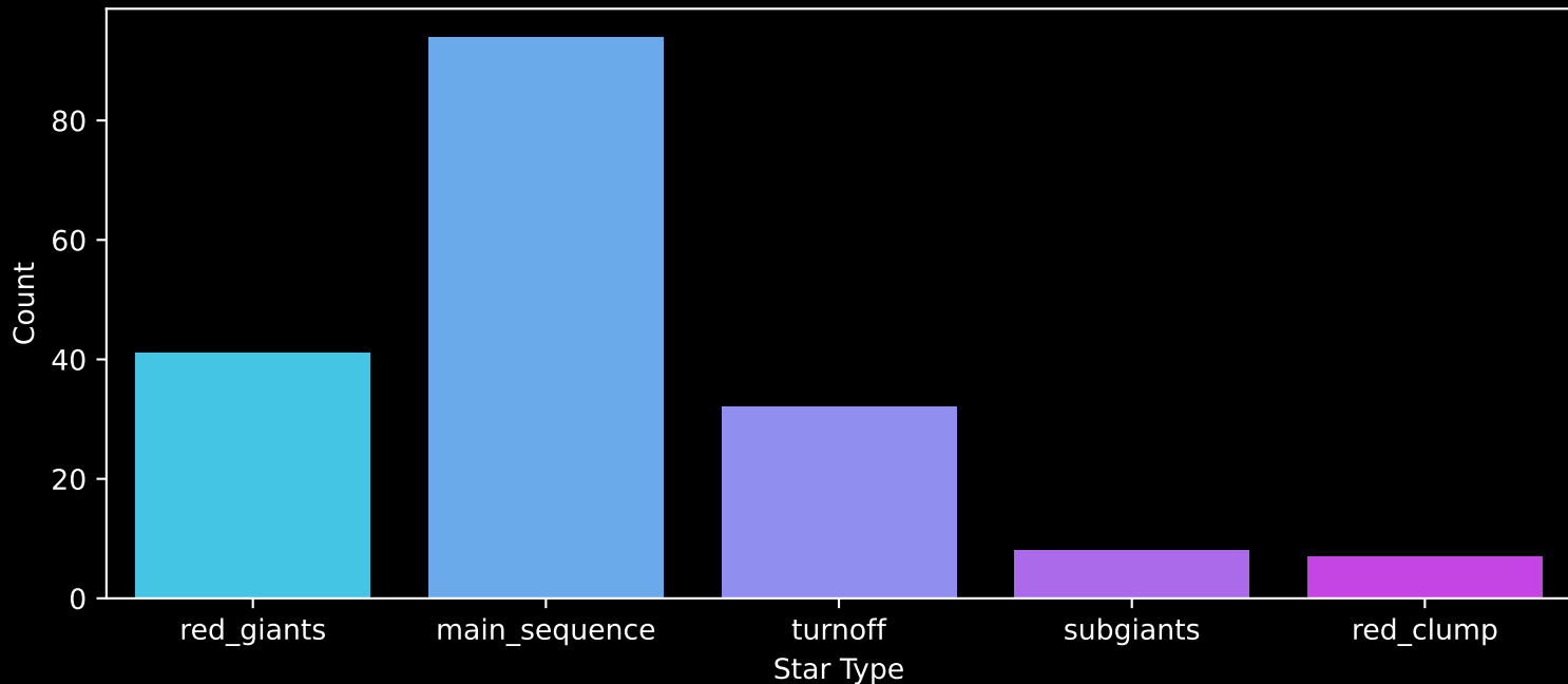
APOGEE DR17 Field: [037+79_MGA] Count plot of Star Type
