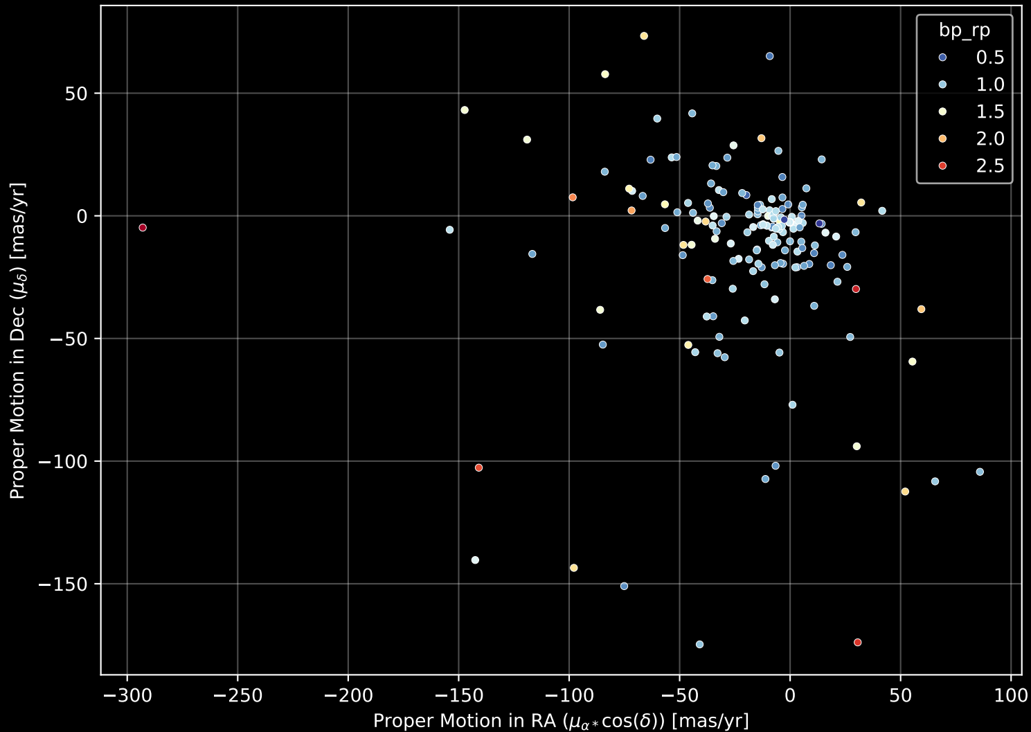
APOGEE DR17 Field: [037+79_MGA] Proper Motion Diagram (n= 182)
