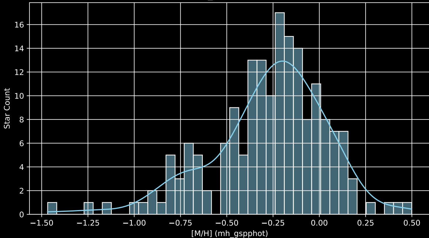
APOGEE DR17 Field: [037+79_MGA [M/H] (mh_gspphot) (n= 179)
